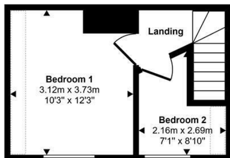
First Floor Approx 20 sq m / 216 sq ft
