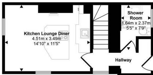
Ground Floor Approx 28 sq m / 299 sq ft
